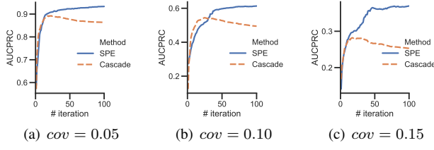
Fig. 5. Training curve under different level of overlap.
